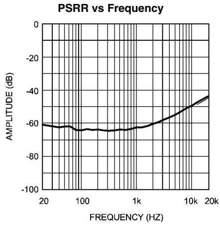
200486g3 Analog V_{DD} = 5V , Digital V_{DD} = 3V R_L = 32\Omega , Vol = 3dB, 44.1kHz Sample Rate
