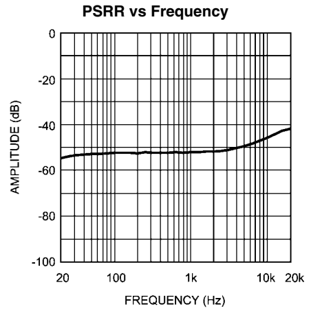
200486e7 Analog V_{DD} = 3V , Digital V_{DD} = 3V R_L = 32\Omega , Vol = 0dB, 44.1kHz Sample Rate
