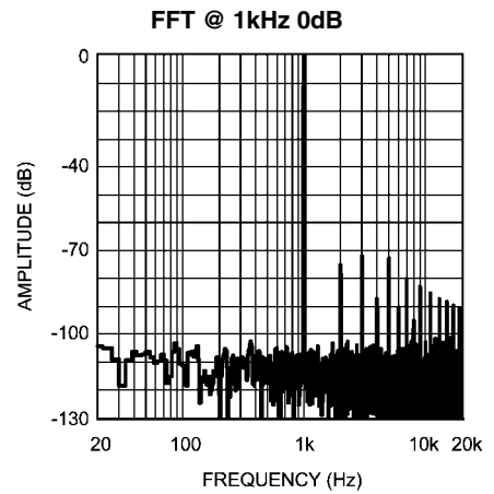
200486f7 Analog V_{DD} = 3V , Digital V_{DD} = 3V R_L = 32\Omega , Vol = 0dB, 44.1kHz Sample Rate
