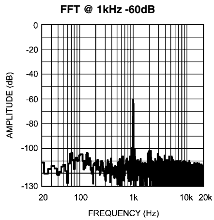
200486d1 Analog V_{DD} = 5V , Digital V_{DD} = 3V R_L = 32\Omega , Vol = 3dB, 44.1kHz Sample Rate
