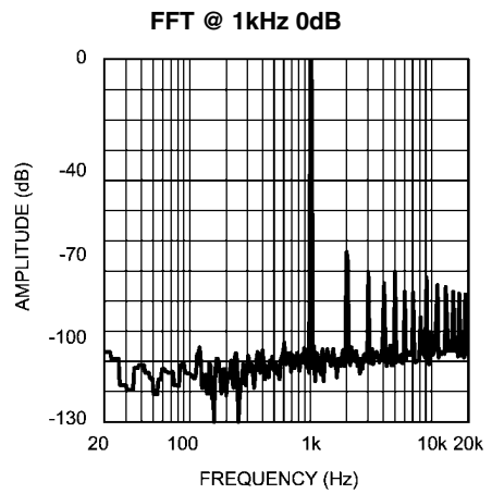
200486c9 Analog V_{DD} = 5V , Digital V_{DD} = 3V R_L = 32\Omega , Vol = 3dB, 44.1kHz Sample Rate
