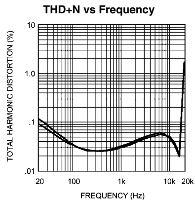
200486g5 Analog V_{DD} = 3V , Digital V_{DD} = 3V R_L = 32\Omega , Power Level = 12mW R & L Channels Shown, 44.1kHz Sample Rate
